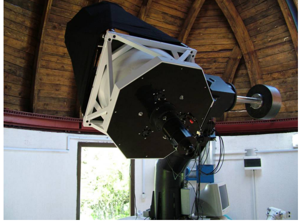
Fig. 1. The 60 cm ASV telescope.
